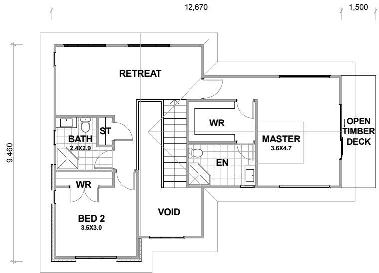
UPPER FLOOR AREA: 89.0 SQM
