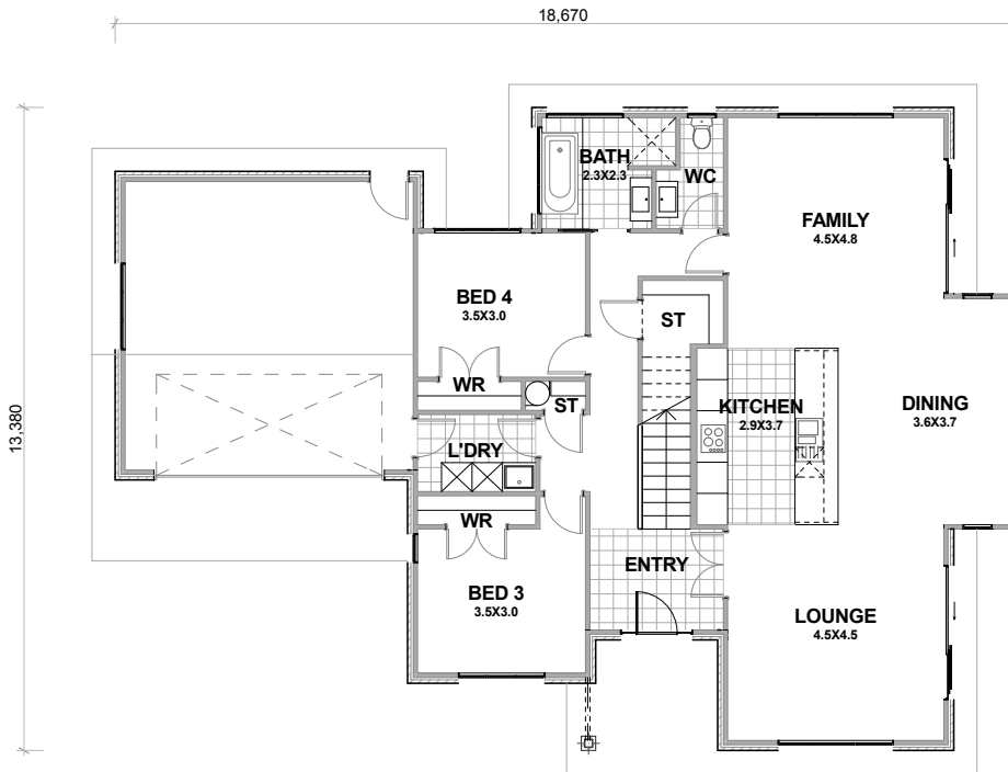
GROUND FLOOR AREA: 180.2 SQM
